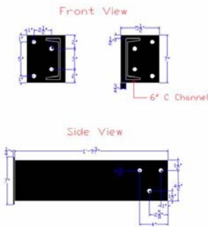
C Channel Diagram
